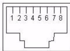
Figure 124 WAN Port Cable Pin Assignments
